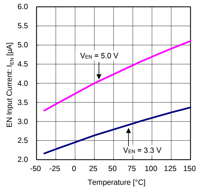
Figure 18. EN Input Current vs Temperature
