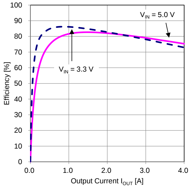
Figure 36. Efficiency vs Output Current ( V_{OUT} = 1.0\text{ V} )
