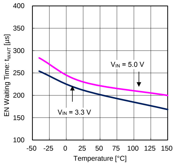
Figure 16. EN Waiting Time vs Temperature
