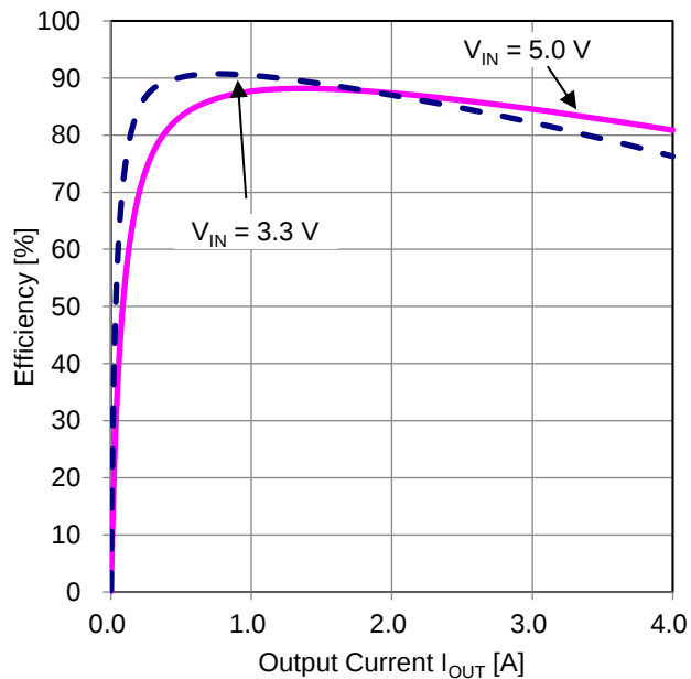
Figure 38. Efficiency vs Output Current ( V_{OUT} = 1.8\text{ V} )
