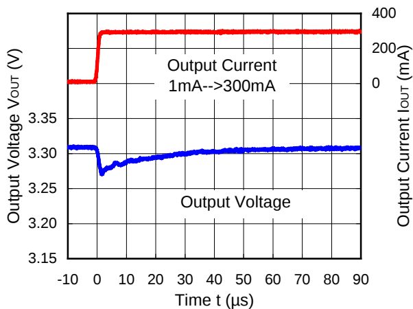
RP505K001C ( V_{IN}=5.0V , V_{OUT}=3.3V ) MODE="H" forced PWM
