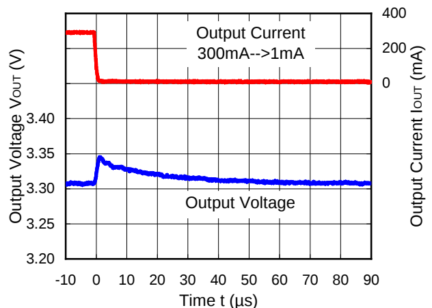
RP505K001C ( V_{IN}=5.0V , V_{OUT}=3.3V ) MODE="H" forced PWM
