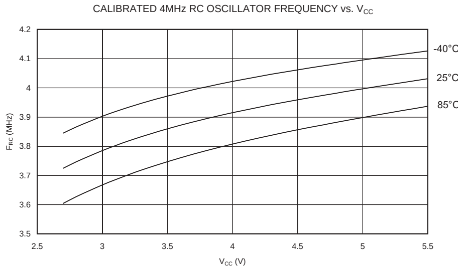
Figure 174. Calibrated 4 MHz RC Oscillator Frequency vs. V CC
