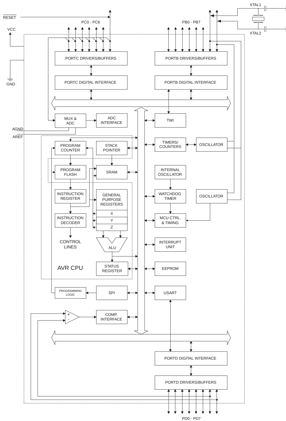
Figure 1. Block Diagram
