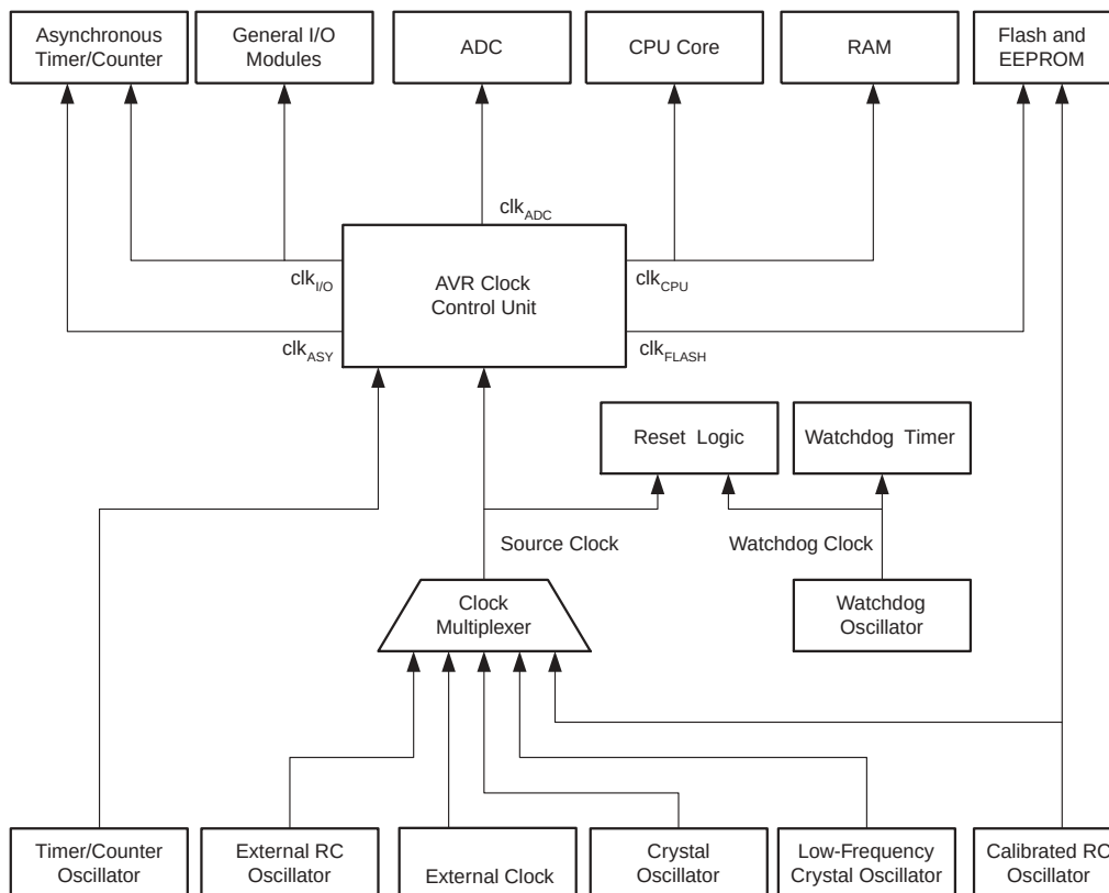
Figure 10. Clock Distribution
