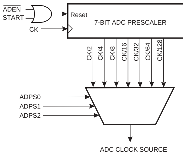
Figure 91. ADC Prescaler
