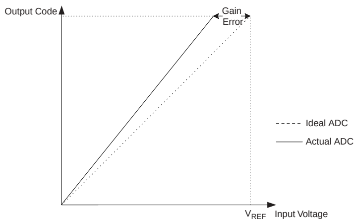
Figure 98. Gain Error
