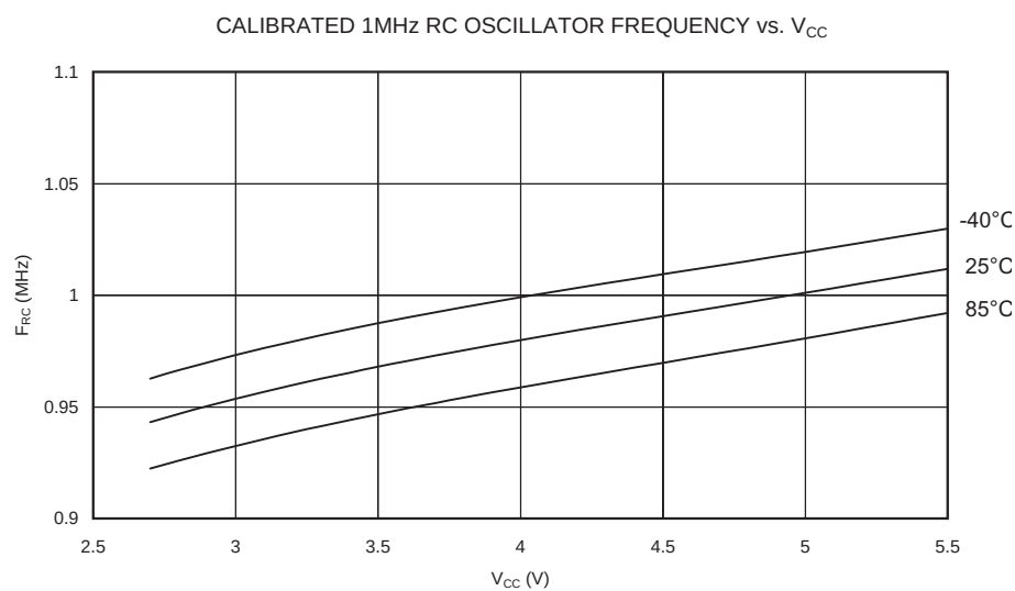
Figure 180. Calibrated 1 MHz RC Oscillator Frequency vs. V_{CC}
