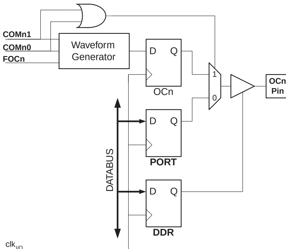
Figure 48. Compare Match Output Unit, Schematic
