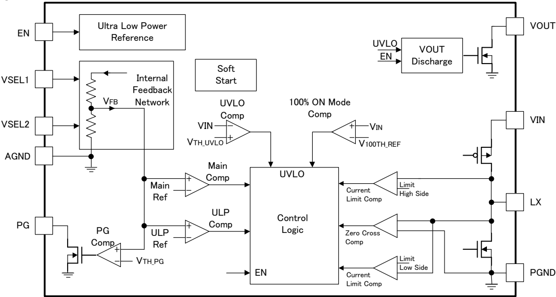
Figure 3. Block Diagram
