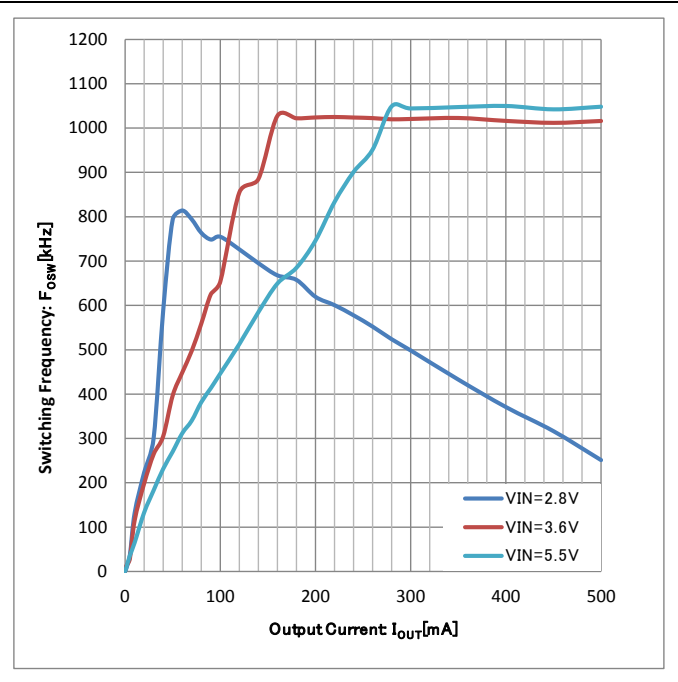
Figure 17. Switching Frequency vs Output Current (VOUT=2.5V)
