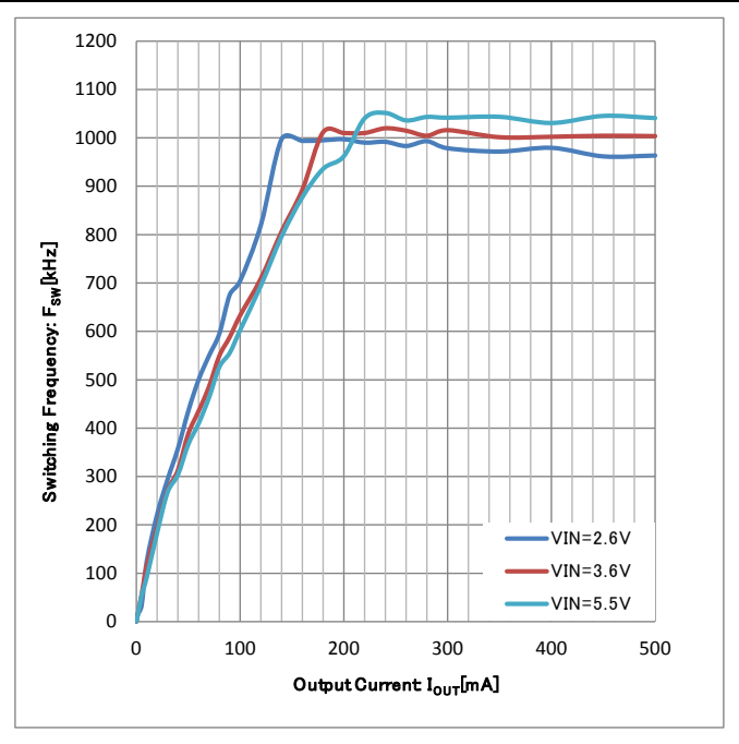
Figure 15. Switching Frequency vs Output Current (VOUT=1.2V)
