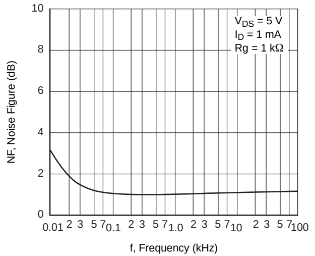
Figure 10. NF – f
