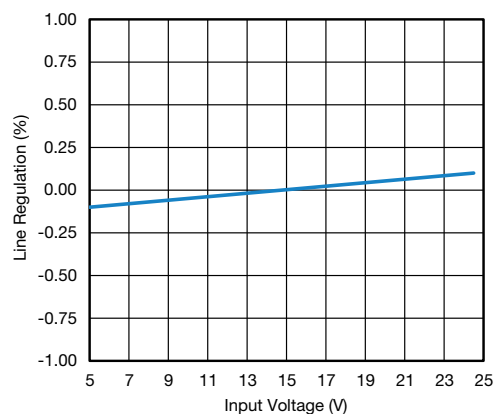
Fig. 19 - Line Regulation vs. Input Voltage
