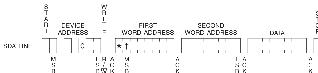
Figure 2. Byte Write
