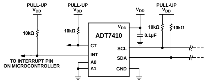
Figure 14. Typical I²C Interface Connection
