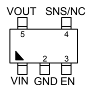
SC-70-5
