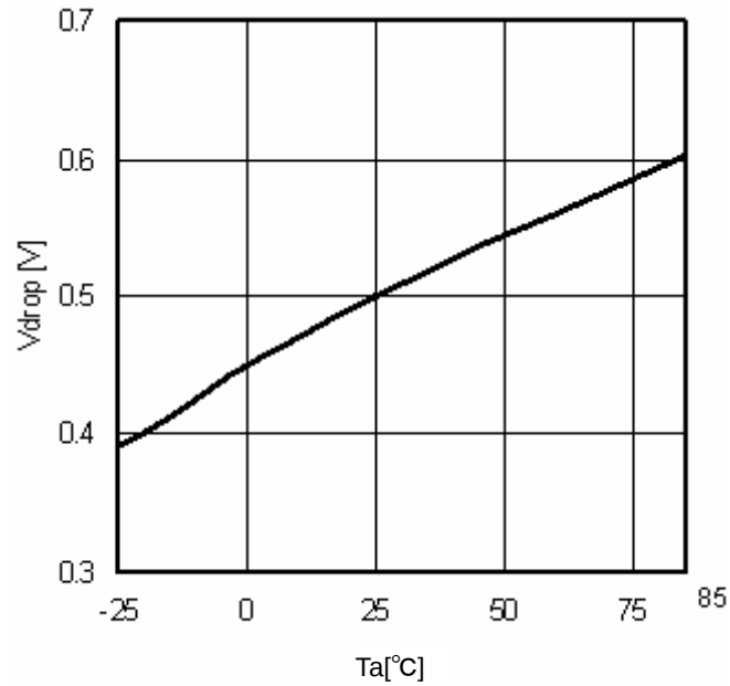
Fig.18 Minimum dropout Voltage 1 ( V_{CC}=5\text{V} , I_O=-1.0\text{A} )
