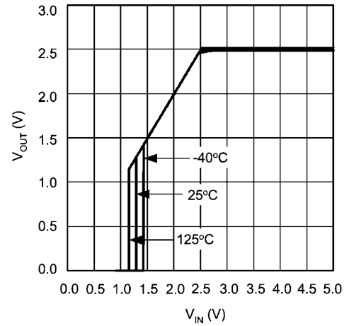
V IN vs V OUT Over Temperature
