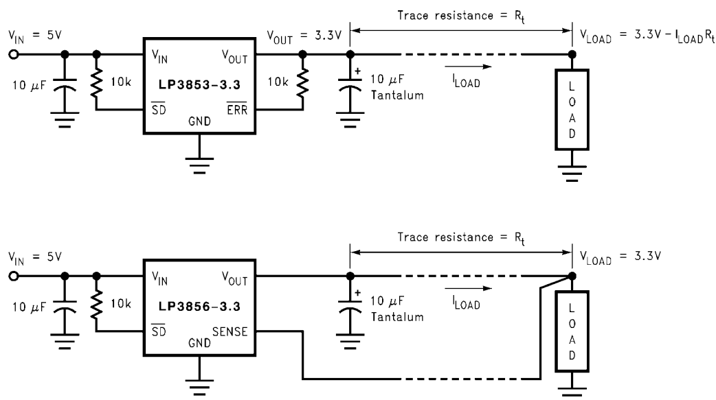
FIGURE 4. Improving remote load regulation using LP3856
