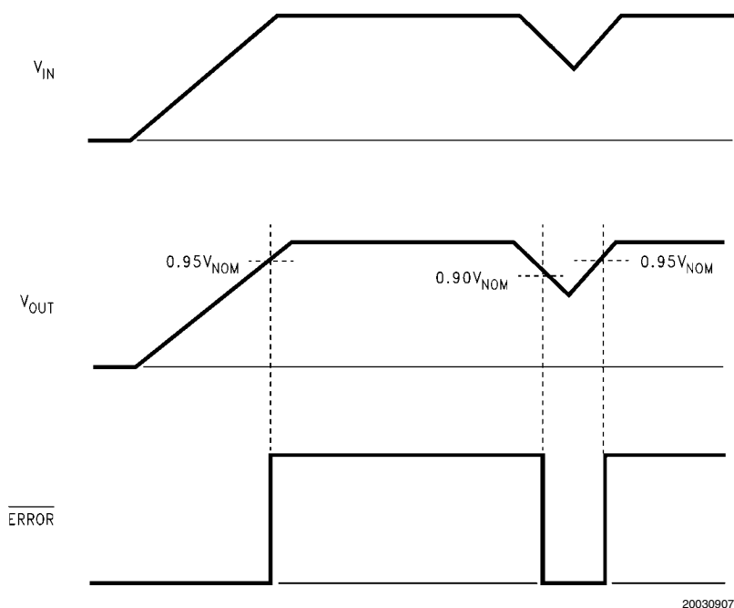
FIGURE 3. \overline{\text{Error}} Flag Operation
