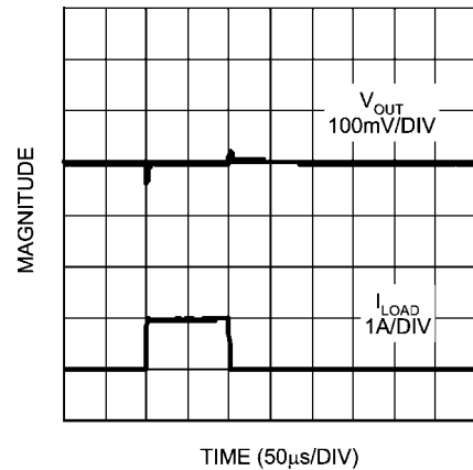
Load Transient Response C IN = C OUT = 100μF, POSCAP
