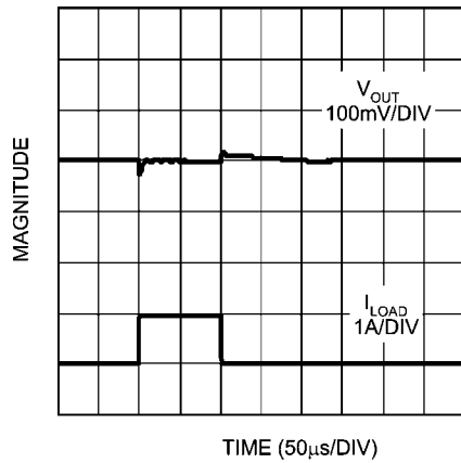
Load Transient Response C IN = C OUT = 100μF, OSCON
