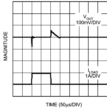
Load Transient Response C IN = C OUT = 10μF, OSCON
