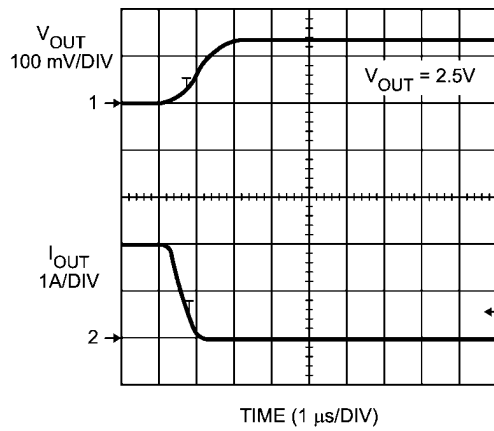
Load Transient Response C_{IN} = 4 \times 10\mu F CERAMIC C_{OUT} = 3 \times 10\mu F CERAMIC
