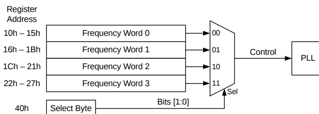
Figure 2. Frequency Words
