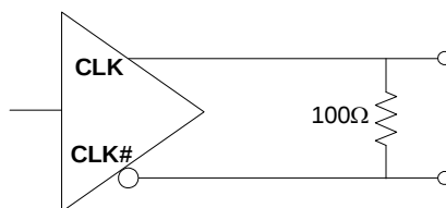
Figure 13. LVDS Termination
