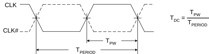
Figure 10. Duty Cycle Timing
