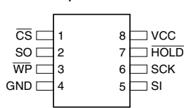
8-pin SOIC
