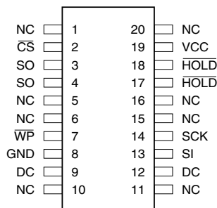
20-lead TSSOP*
