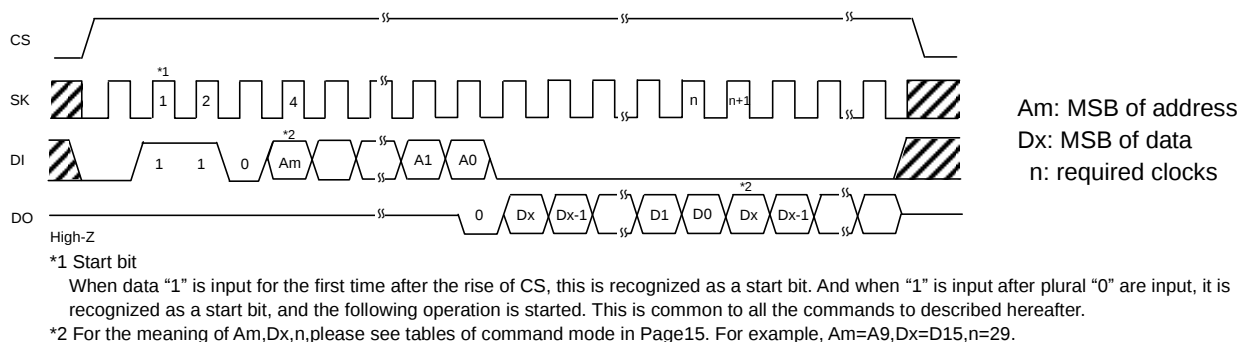
Figure 35. Read cycle
