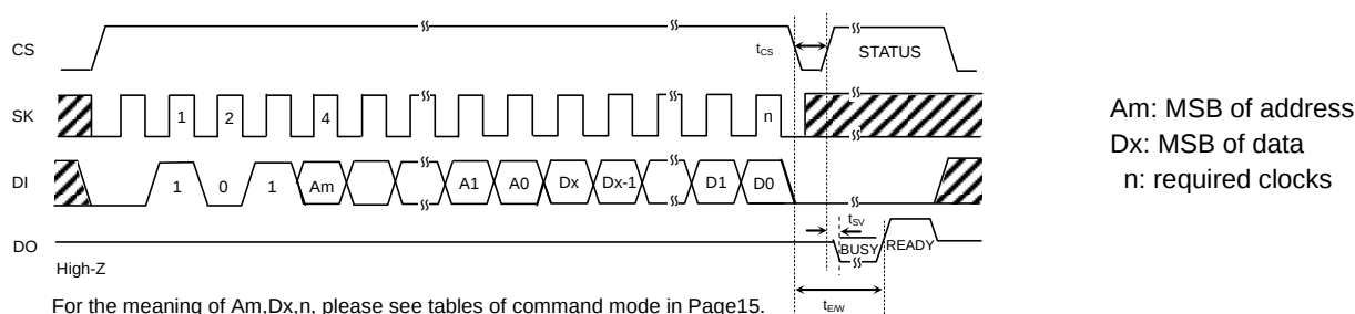
Figure 36. Write cycle
