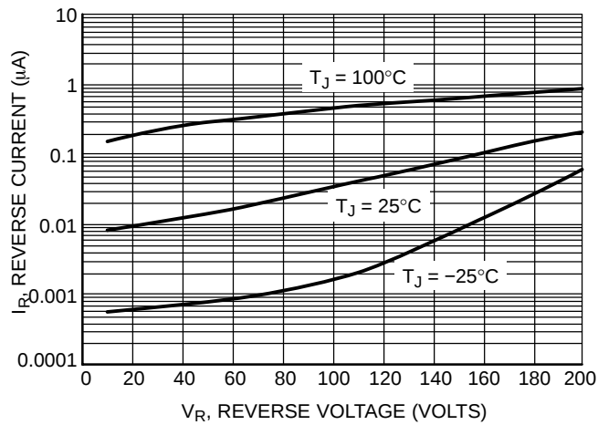
Figure 11. Typical Reverse Current
