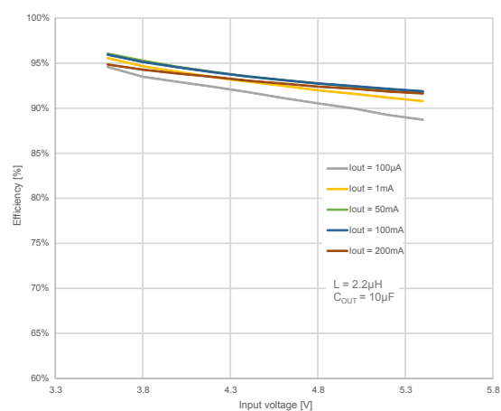
Figure 7. Efficiency vs V_{IN} , V_{OUT} = 3.3\text{ V}
