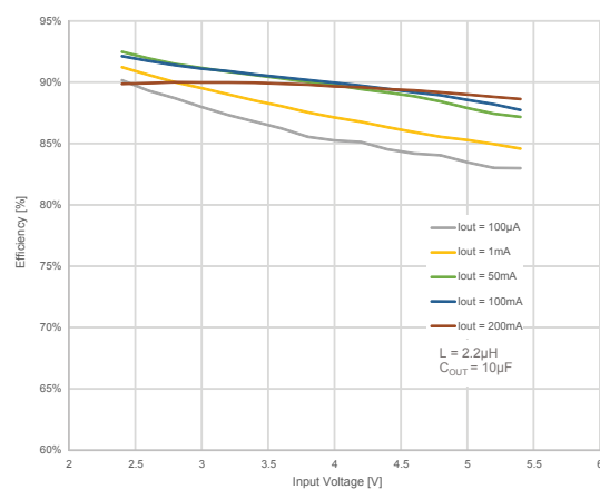
Figure 5. Efficiency vs V_{IN} , V_{OUT} = 1.8\text{ V}
