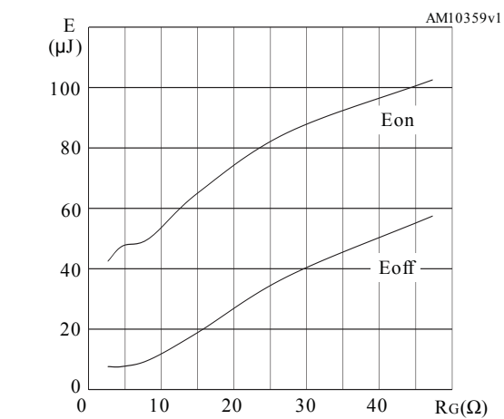
Figure 13. Switching energy vs gate resistance
