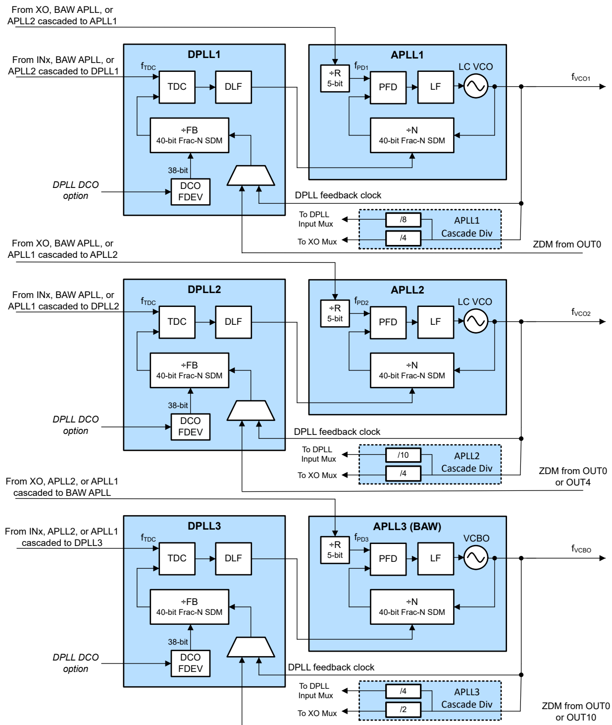
Figure 8-2. PLL Architecture
