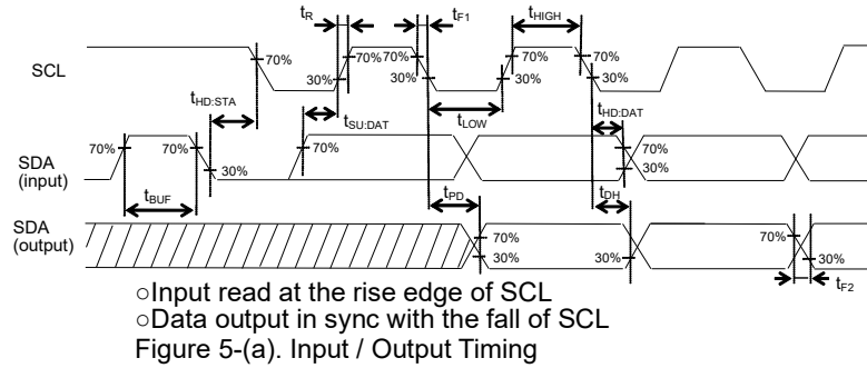
Figure 5-(a). Input / Output Timing
