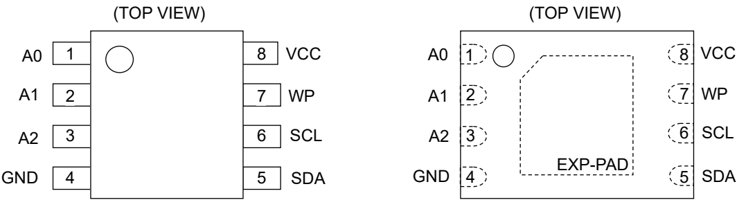
Figure 3-(a). Pin Configuration (SOP8 *1 , SOP-J8, TSSOP-B8, MSOP8) *1 Last Time Buy.
