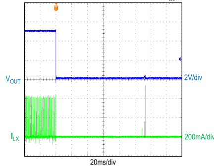
SHORT-CIRCUIT PROTECTION 5V OUTPUT, LOAD SHORT-TO-GROUND FIGURE 11 CIRCUIT
