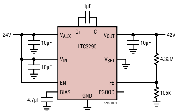
Figure 8. 24V to 42V Boost
