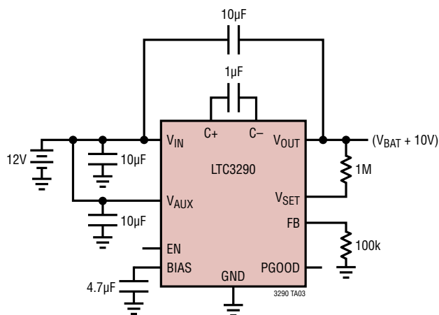
Figure 7. 10V Plus Battery Tracking Application
