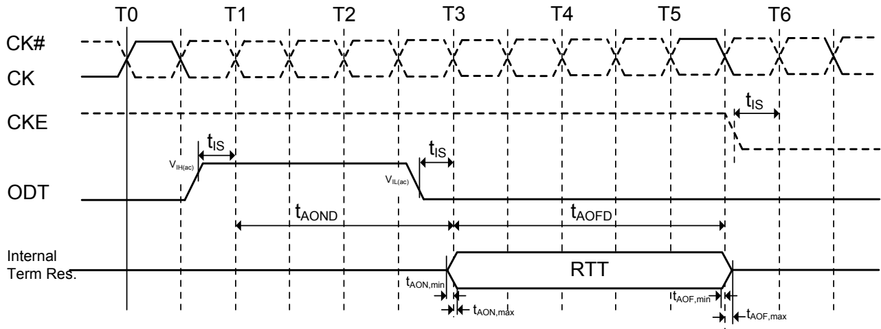
Figure 15. ODT timing for active standby mode
