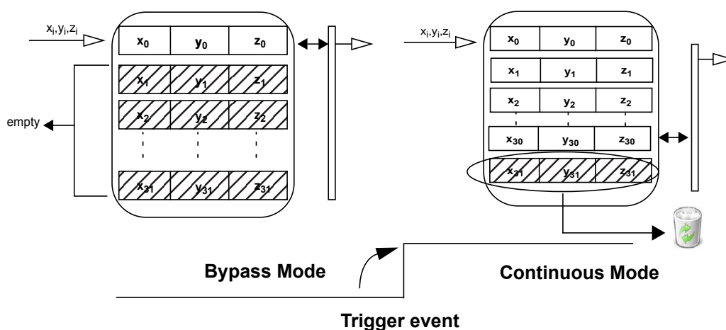
Figure 10. Bypass-to-continuous mode
