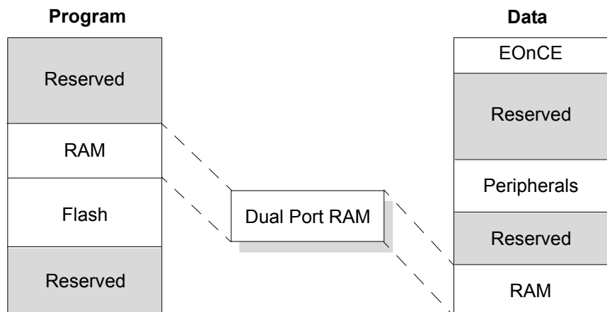
Figure 4-2 Dual Port RAM for 56F8027
