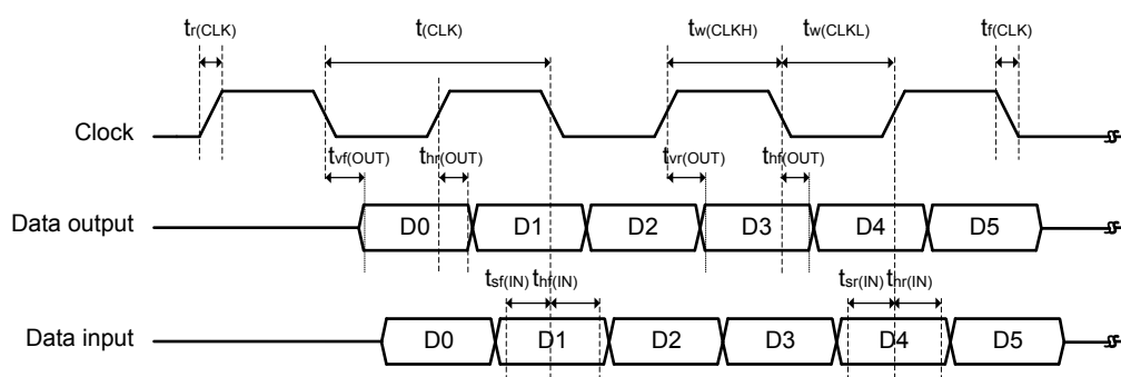
Figure 50. OctoSPI timing diagram - DTR mode
