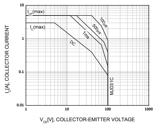
Figure 6. Safe Operating
