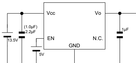
Measurement setup for Figure 28, 39, 51 and 63
