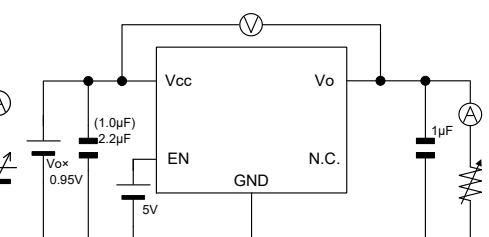
Measurement setup for Figure 40, 52 and 64
