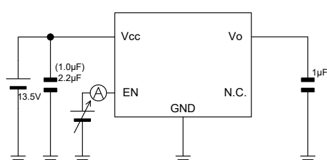
Measurement setup for Figure 32, 44, 56 and 68
