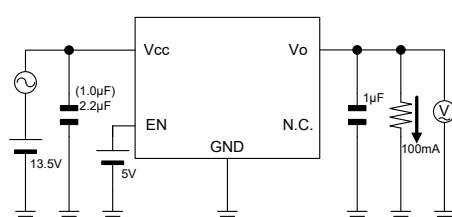
Measurement setup for Figure 27, 38, 50 and 62
