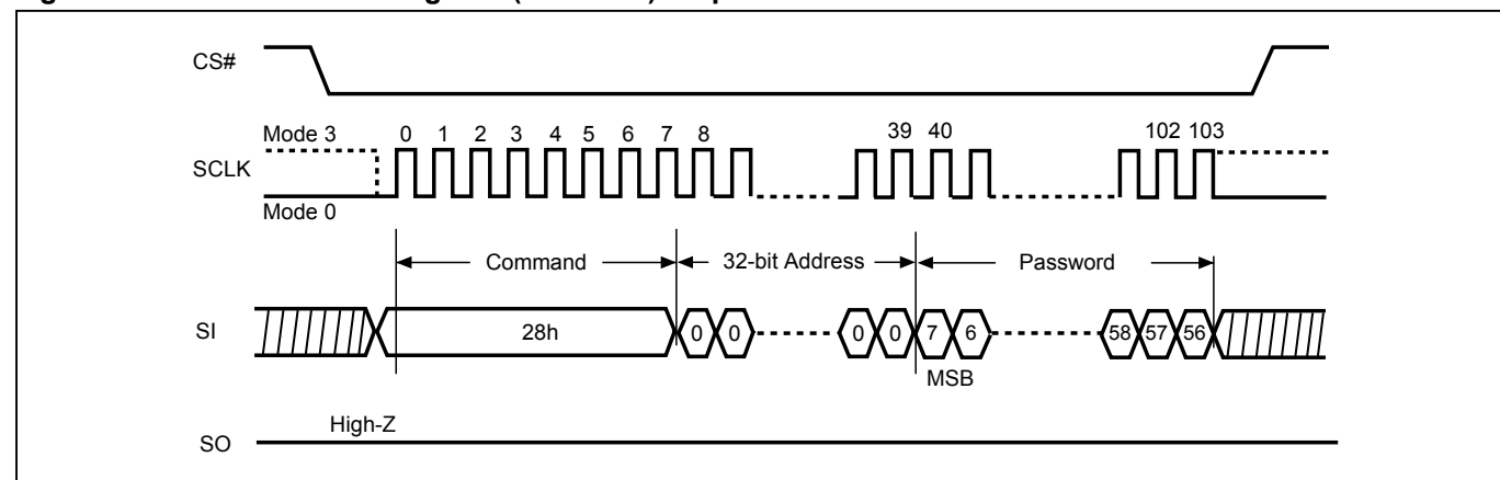
Figure 93. Write Password Register (WRPASS) Sequence
