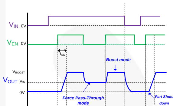
Figure 21. Pass-Through Profile
