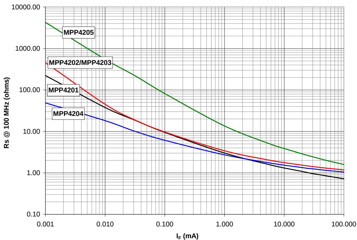
TYPICAL R_S VS I_F @ 25°C
