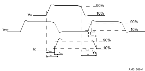
Figure 29. Switching waveform
