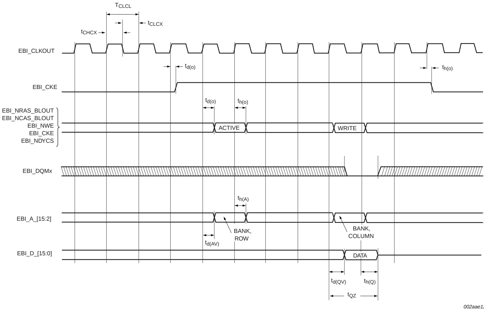
Fig 17. SDRAM bank activate and write timing
