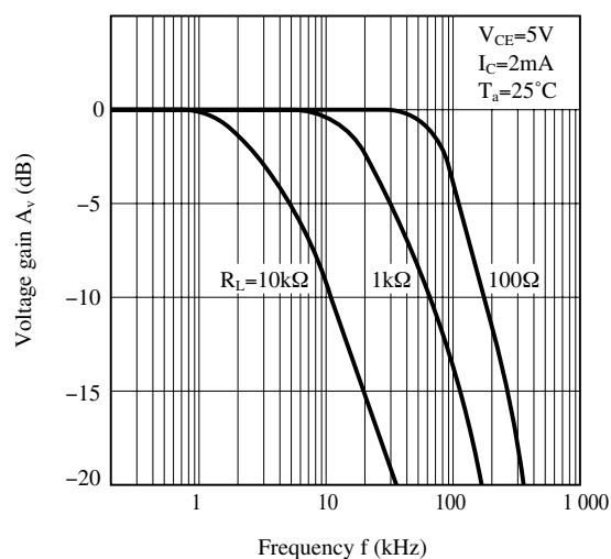
Fig.15 Frequency Response
