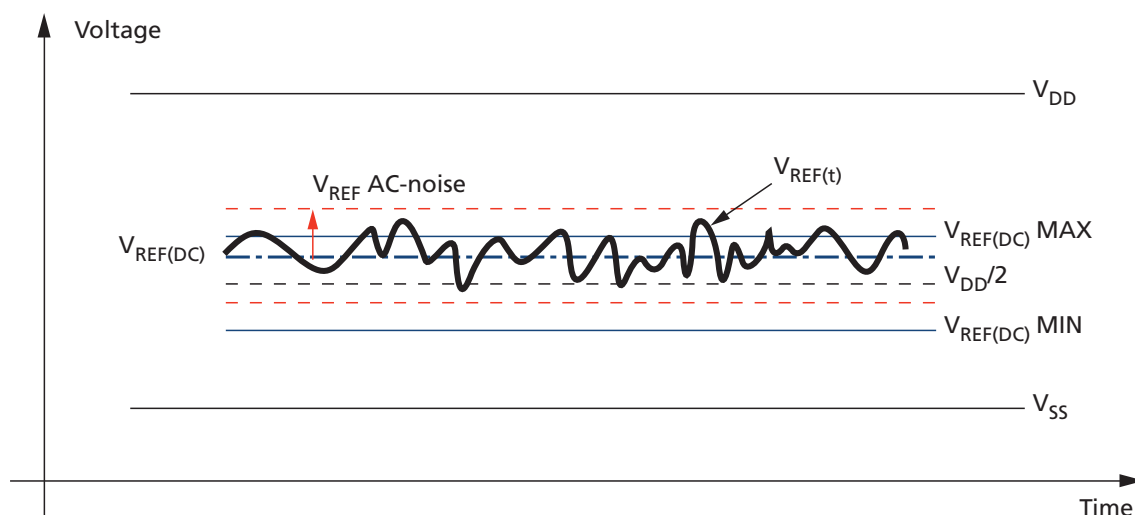
Figure 208: V REFDO Voltage Range
