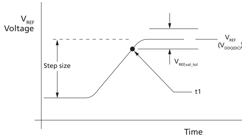
Figure 68: V_{REF} Step: Single Step Size Increment Case
