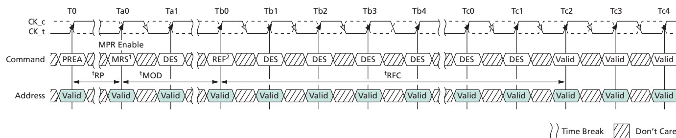
Figure 40: REFRESH Timing
