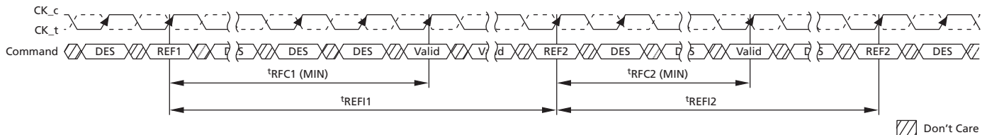
Figure 87: OTF REFRESH Command Timing
