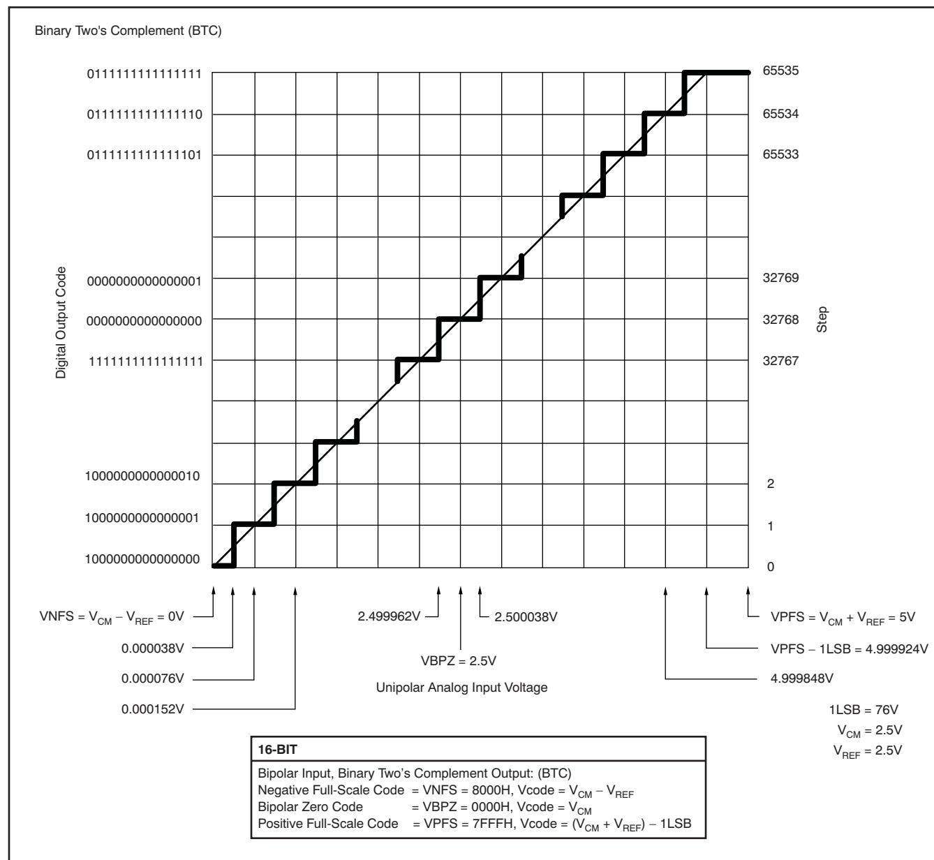
Figure 32. Ideal Conversion Characteristics (Condition: Single-Ended, V_{CM} = 2.5V , V_{REF} = 2.5V )
