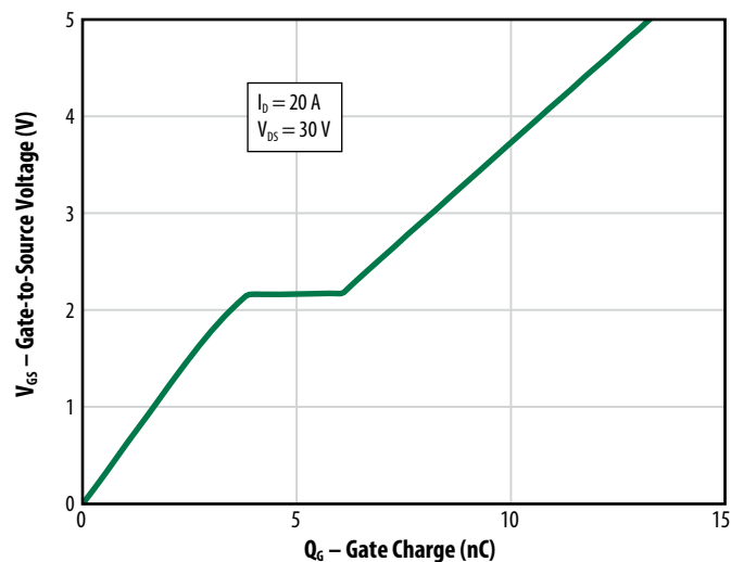
Figure 7b (Q2): Gate Charge
