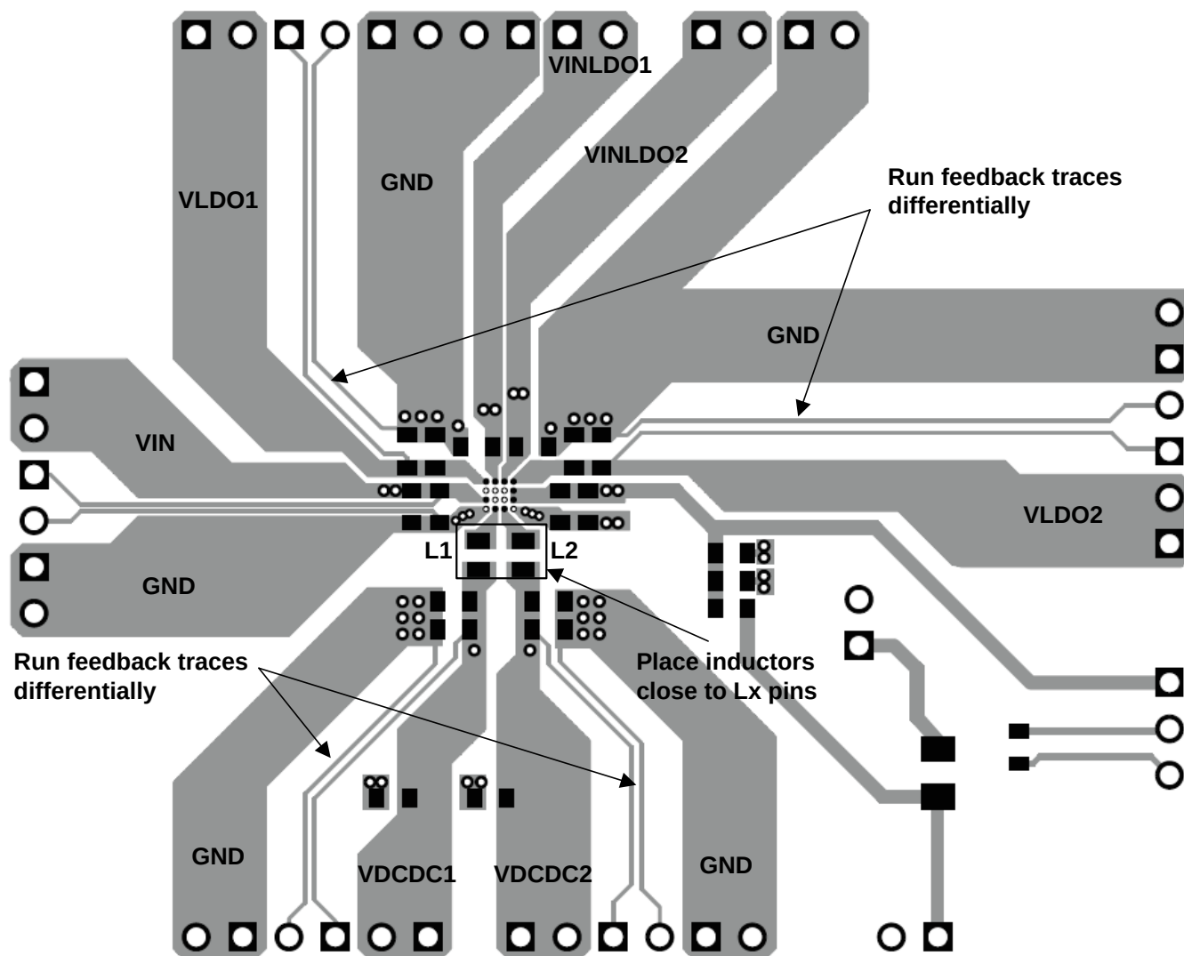
Figure 15. Layout Recommendation
