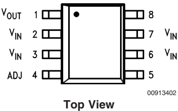
8-Pin SOIC
