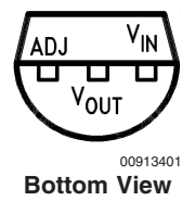
3-Pin TO92
