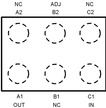
6-Bump micro SMD
