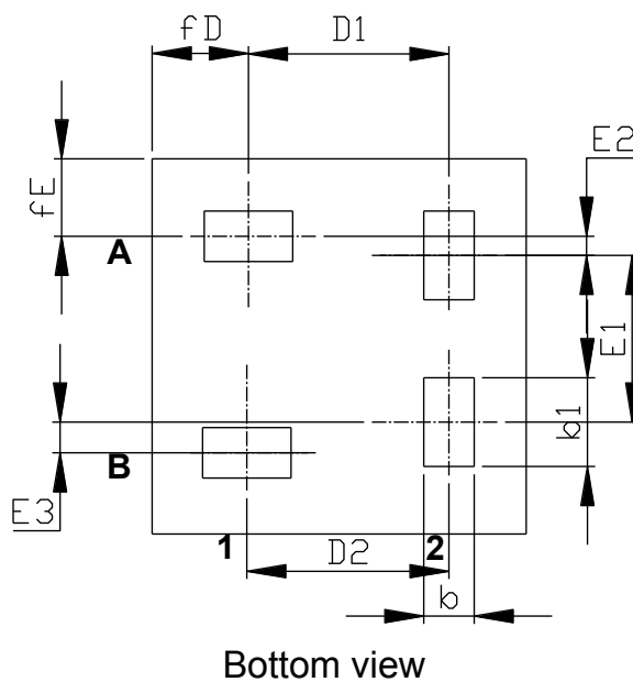
Figure 29. STSTAMP™ (0.47x0.47) mm 2 package outline
