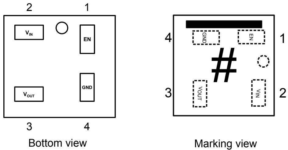
Figure 2. Pin connection
