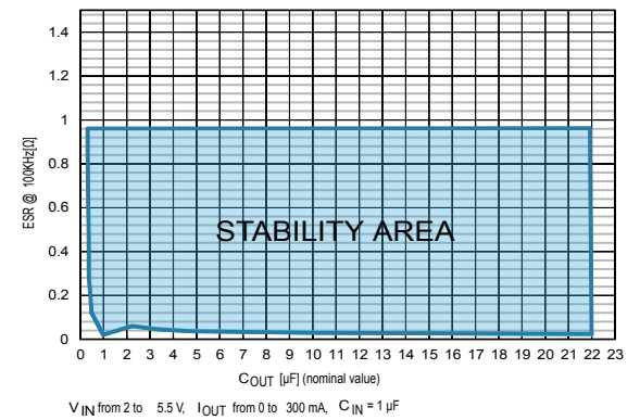
Figure 17. Stability area vs ( C_{OUT} , ESR)
