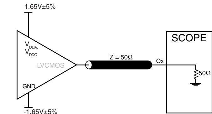
3.3V Output Load AC Test Circuit
