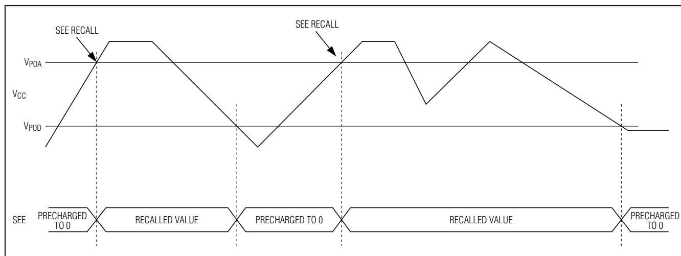
Figure 10. Low-Voltage Hysteresis Example
