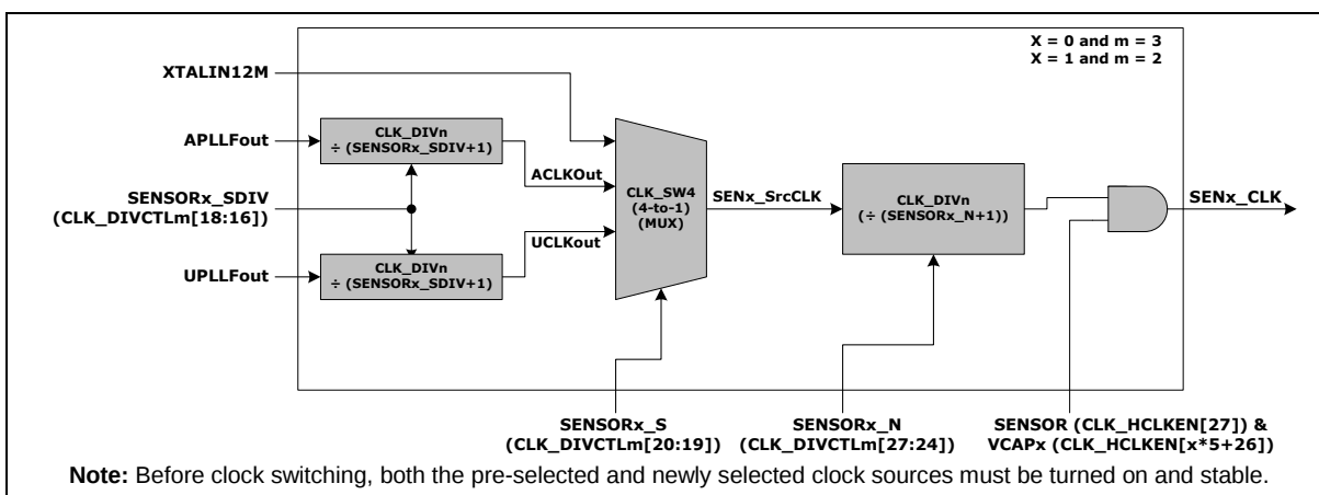
Figure 6.3-9 CMOS Sensor Controller Divider Block Diagram
