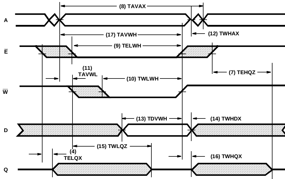
FIGURE 3. WRITE CYCLE 1: CONTROLLED BY \overline{W} (LATE WRITE)
