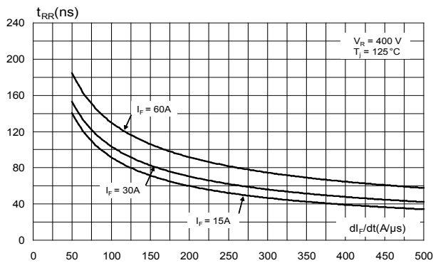
Figure 9. Reverse recovery time versus dl_F/dt (typical values)
