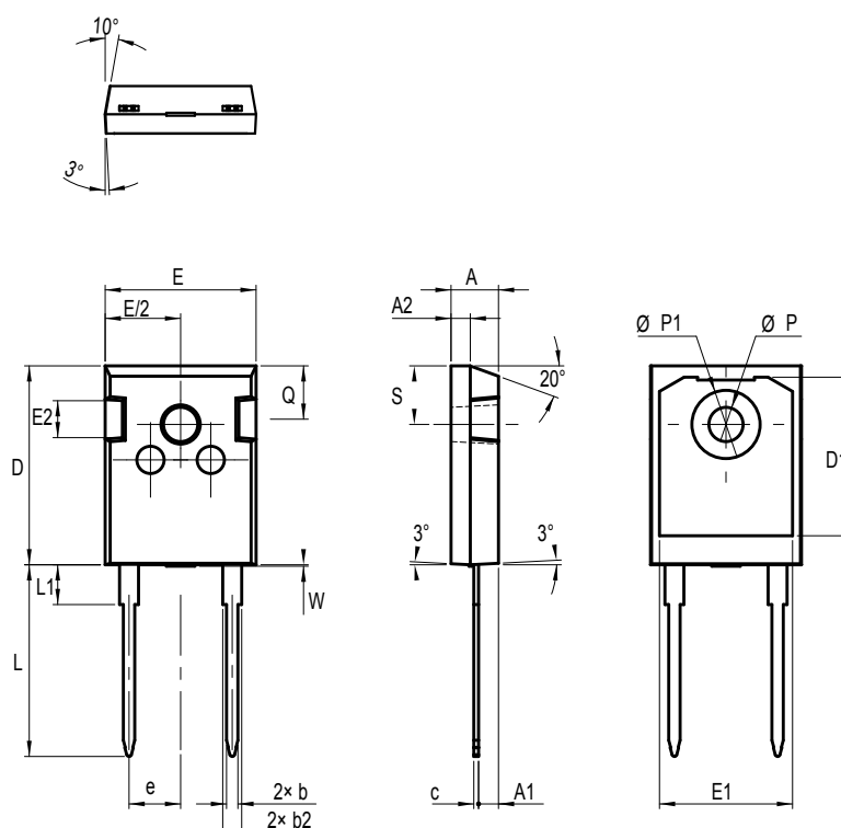
Figure 17. DO-247 LL package outline
