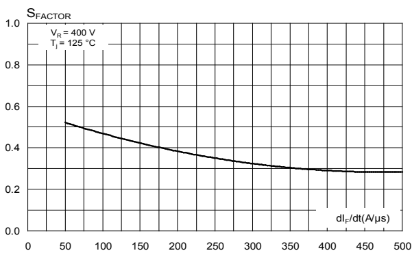
Figure 11. Reverse recovery softness factor versus dl_F/dt (typical values)
