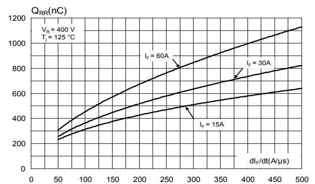
Figure 10. Reverse recovery charges versus dl_F/dt (typical values)
