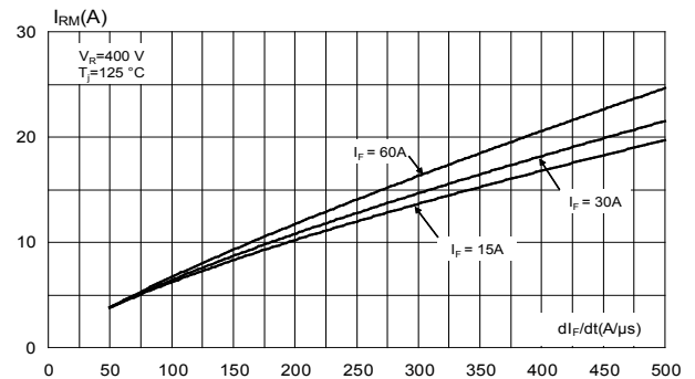
Figure 8. Peak reverse recovery current versus dl_F/dt (typical values)
