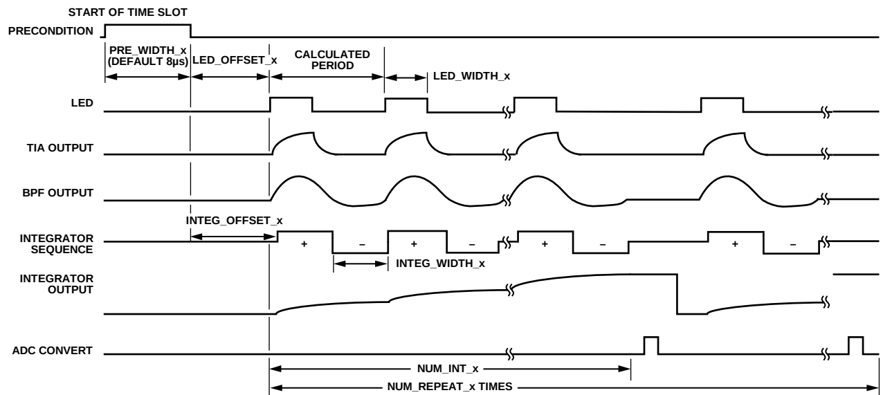
Figure 44. Multiple Integration Mode with LED as Stimulus
