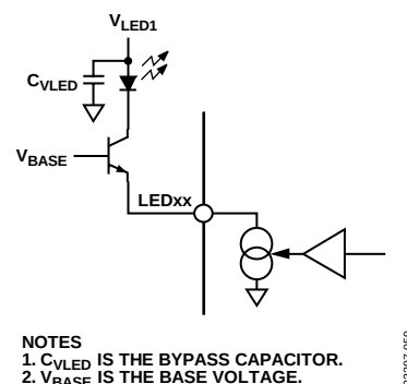
Figure 21. LED Driver Overvoltage Protection Circuit
