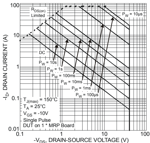
Fig. 14 SOA, Safe Operation Area
