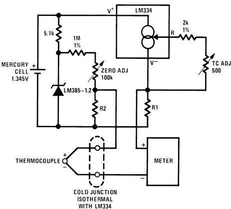
Micropower Thermocouple Cold Junction Compensator
