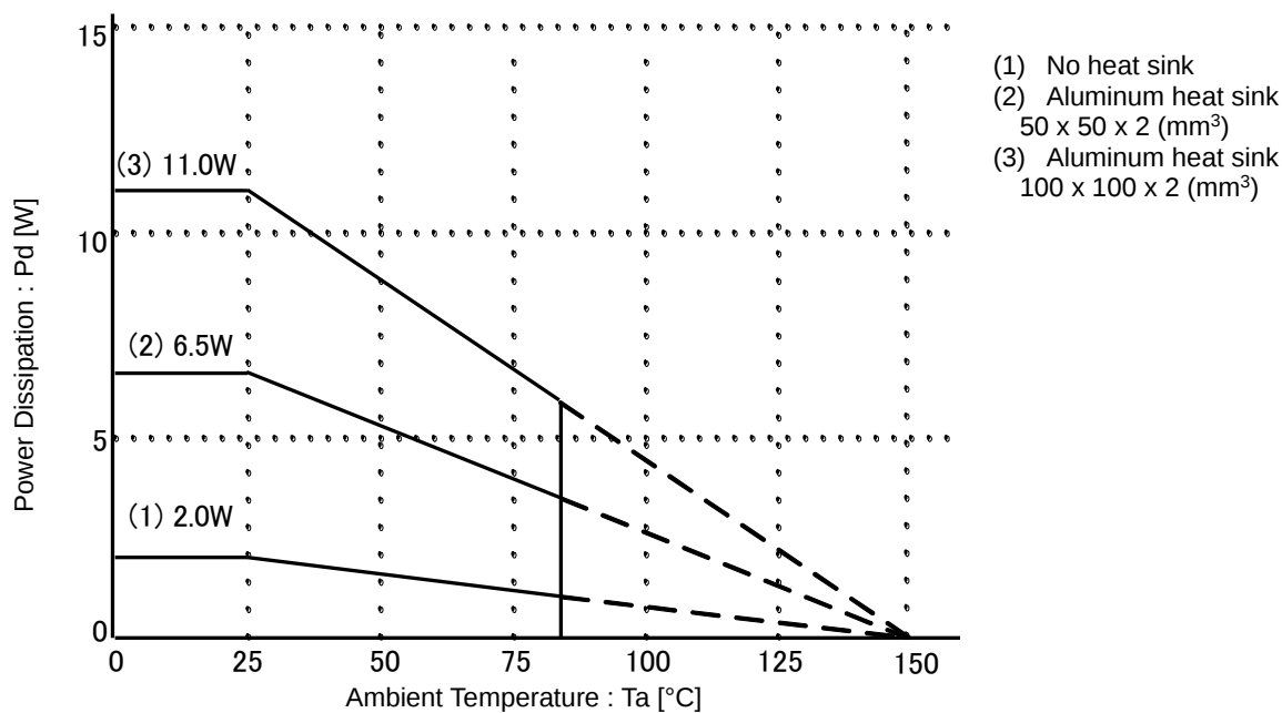
Figure 29. Power Dissipation
