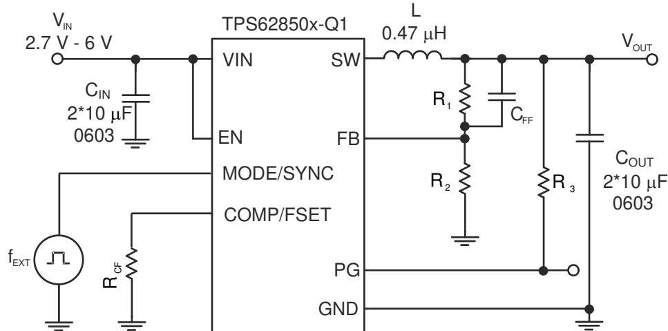
Figure 10-58. Schematic using External Synchronization
