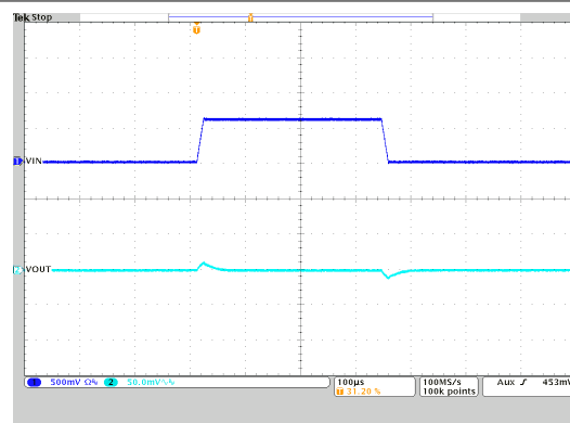
Figure 10-39. Line Transient Response
