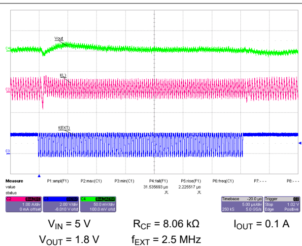
Figure 10-60. Switching from External Synchronization to Internal Fixed Frequency
