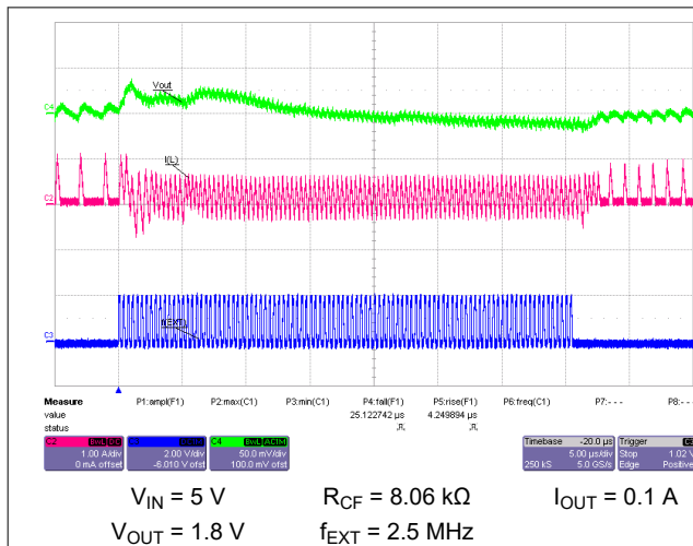
Figure 10-59. Switching from External Synchronization to Power-Save Mode (PFM)
