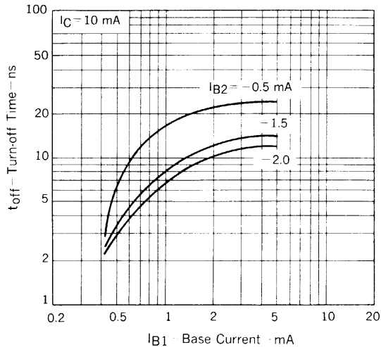
TURN OFF TIME vs. BASE CURRENT
